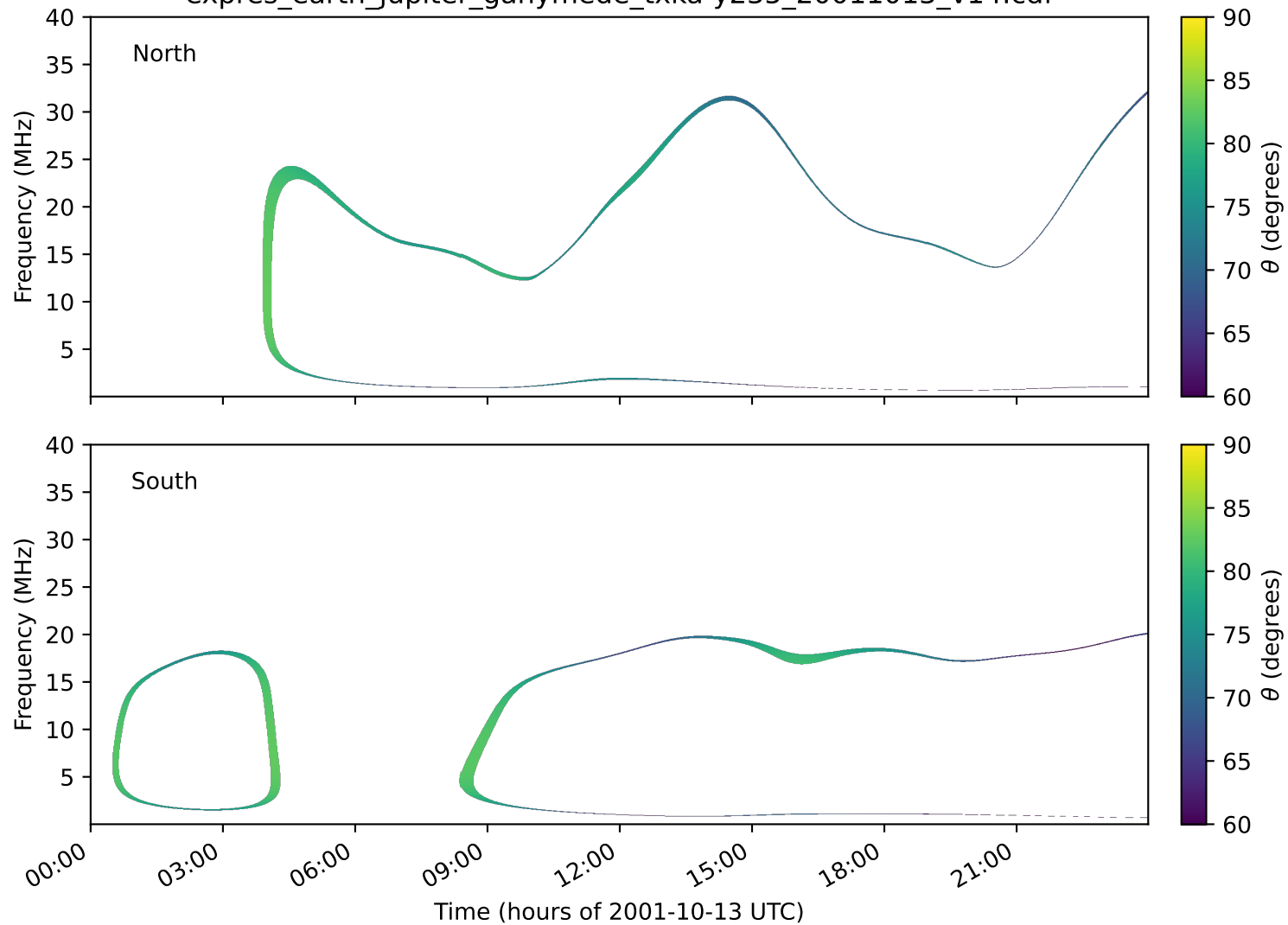
expres_earth_jupiter_ganymede_txka-y235_20011013_v14.cdf
