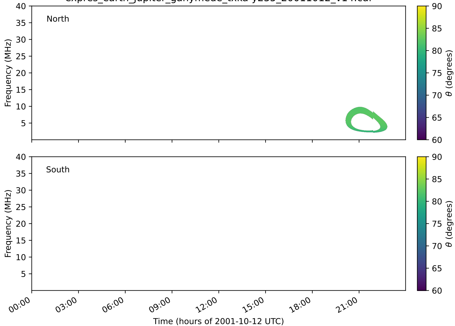
expres_earth_jupiter_ganymede_txka-y235_20011012_v14.cdf
