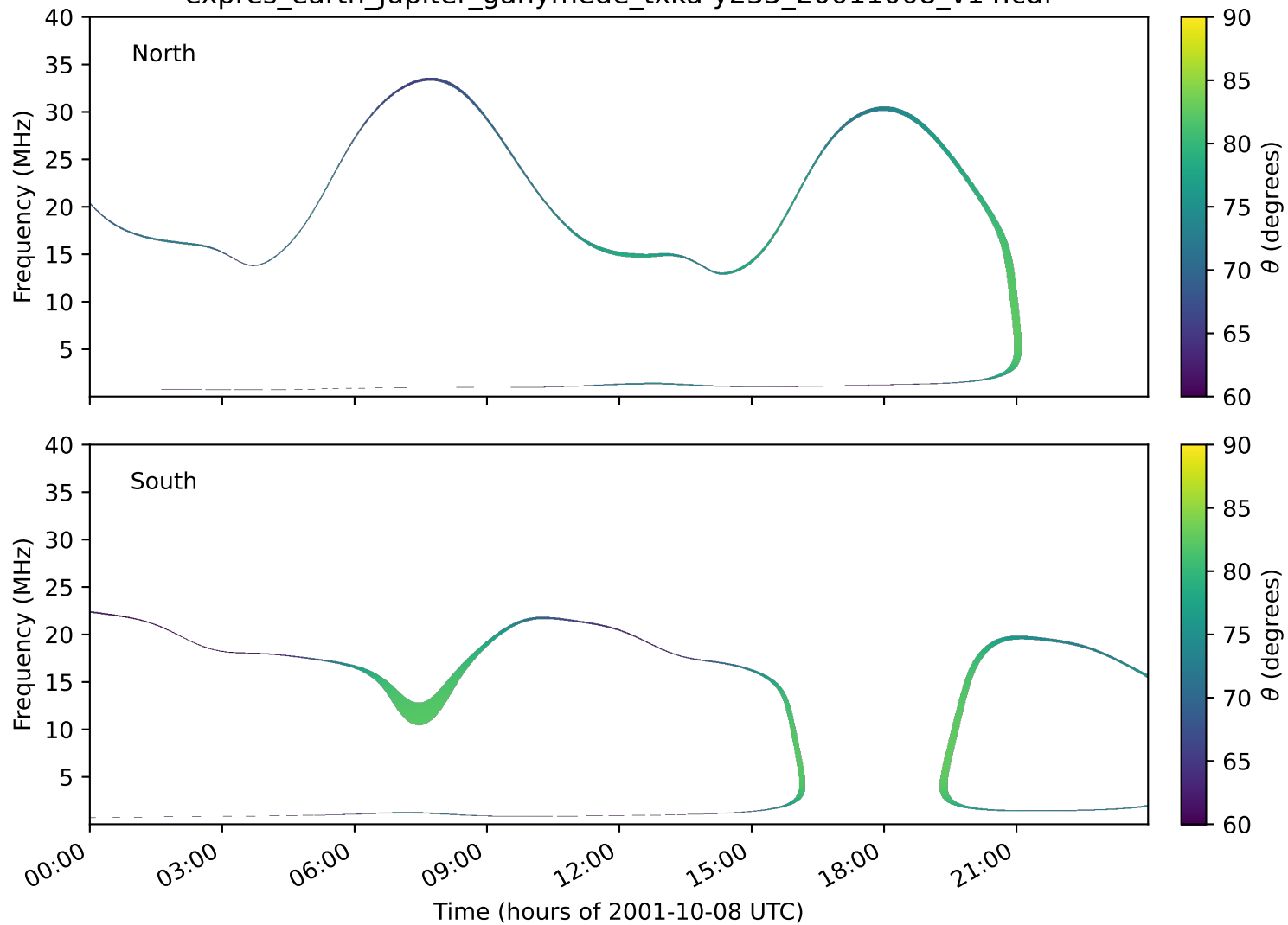
expres_earth_jupiter_ganymede_txka-y235_20011008_v14.cdf
