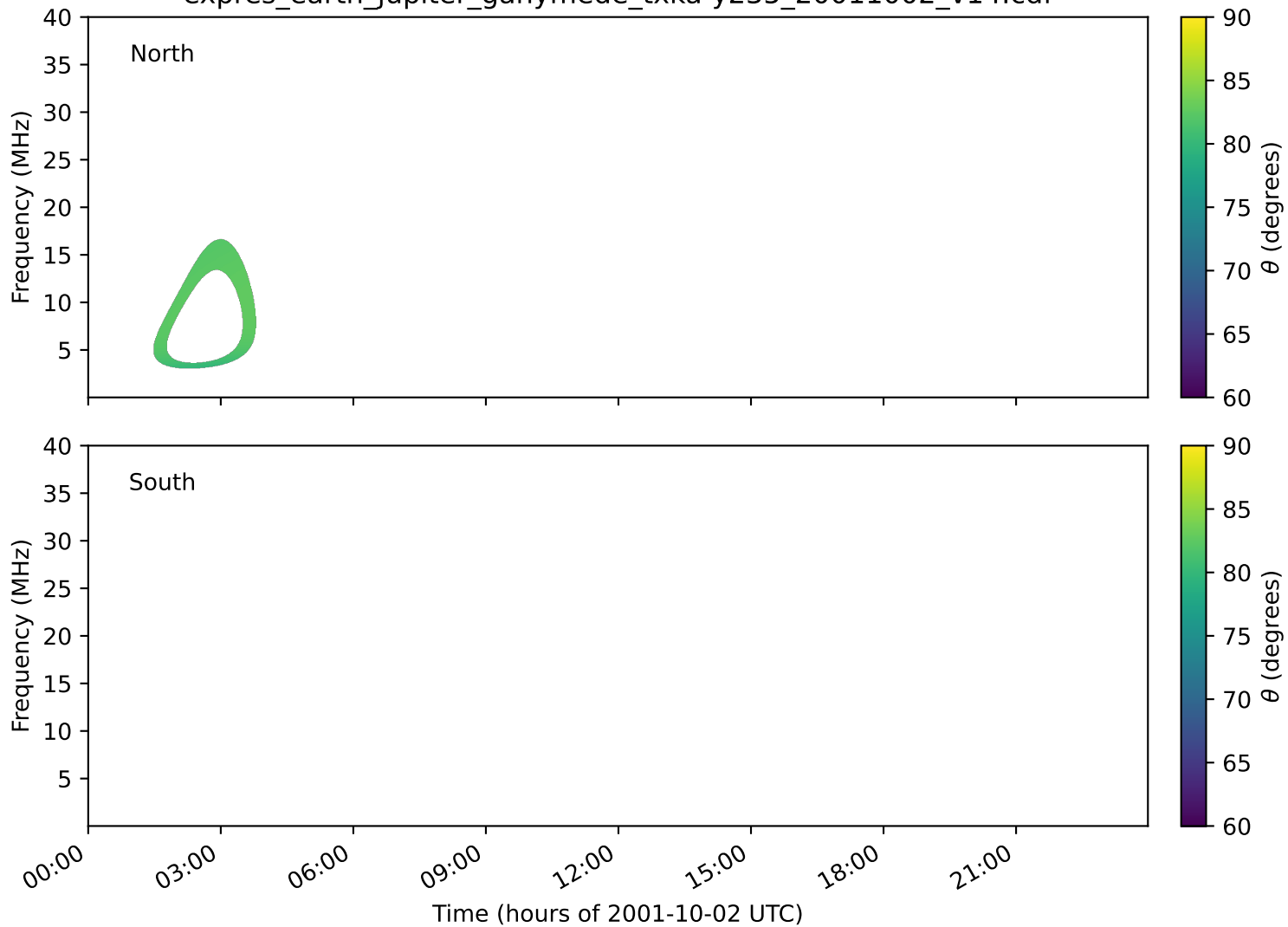
expres_earth_jupiter_ganymede_txka-y235_20011002_v14.cdf
