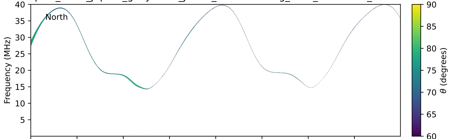
expres_earth_jupiter_ganymede_jrm33_lossc-wid1deg_3kev_20011028_v11.cdf
