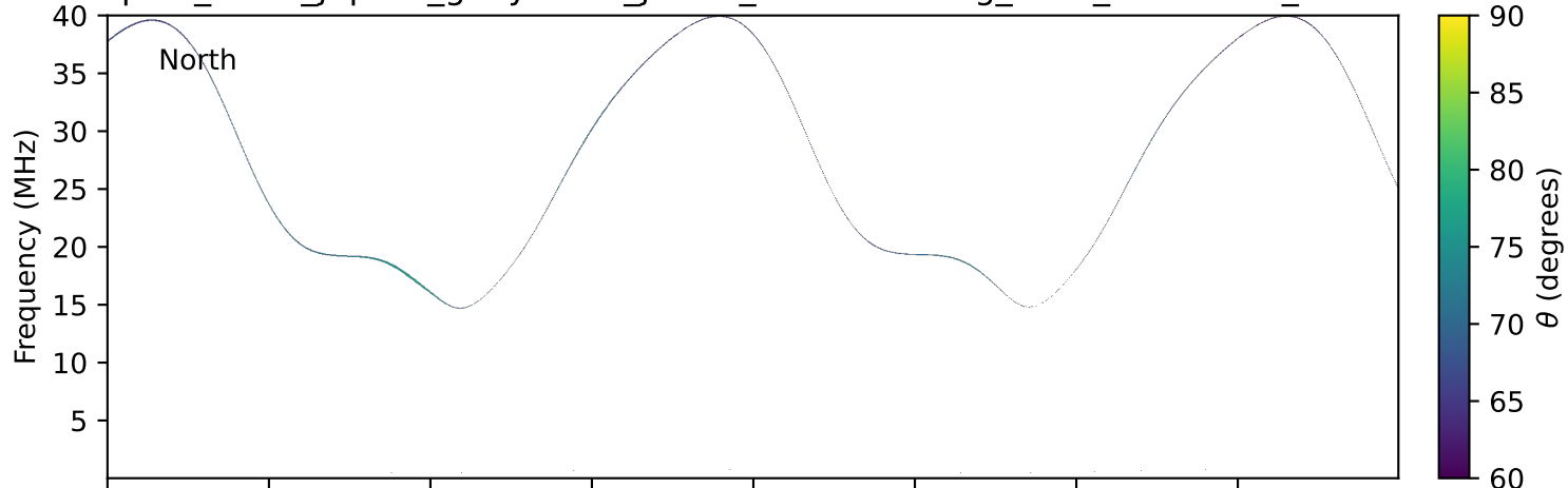
expres_earth_jupiter_ganymede_jrm33_lossc-wid1deg_3kev_20011014_v11.cdf
