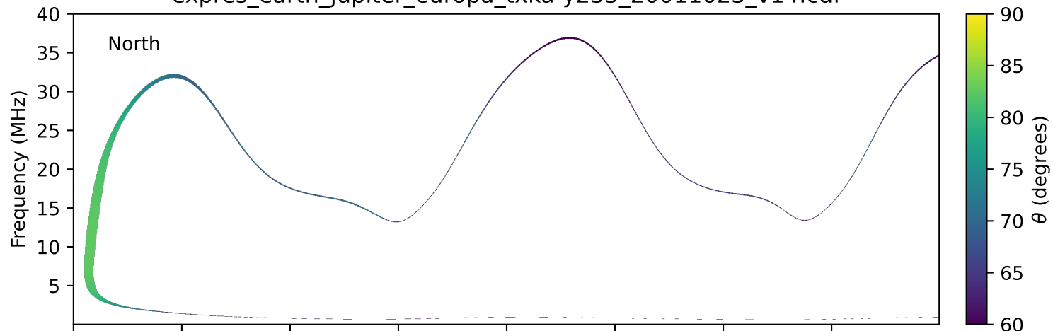
expres_earth_jupiter_europa_txka-y235_20011023_v14.cdf
