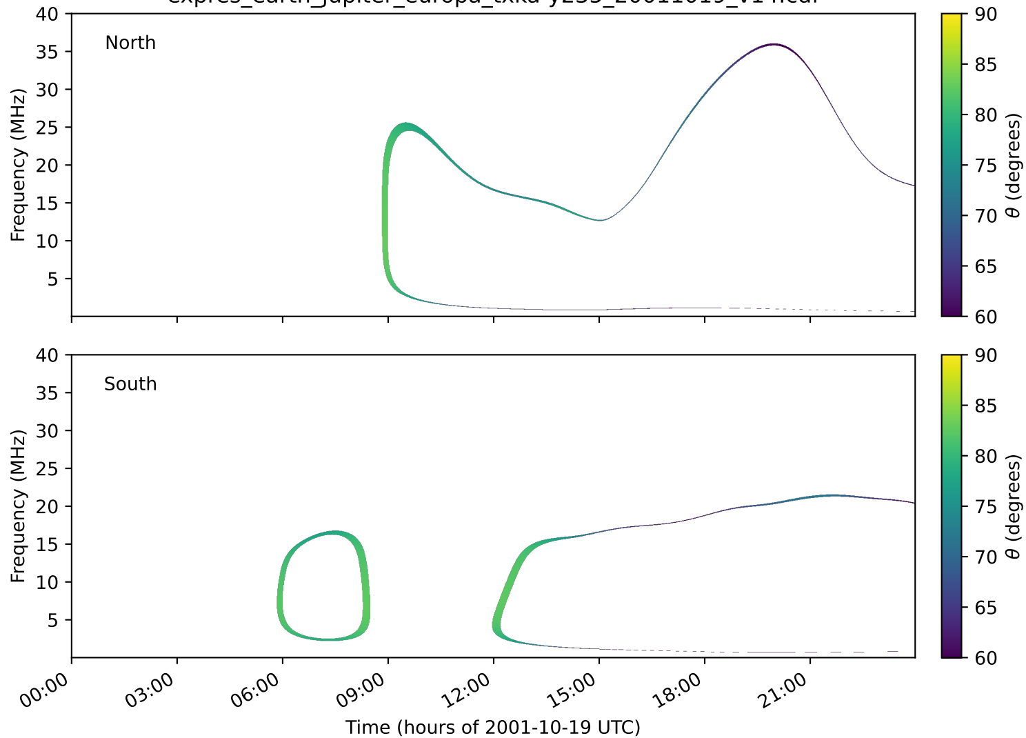
expres_earth_jupiter_europa_txka-y235_20011019_v14.cdf
