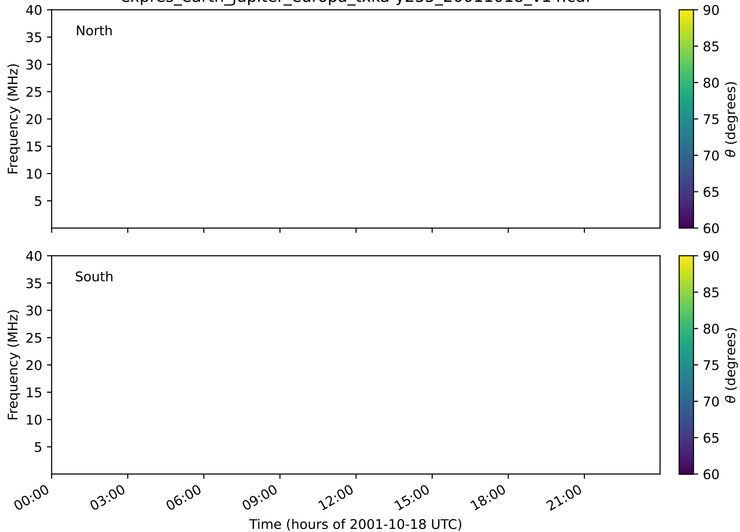
expres_earth_jupiter_europa_txka-y235_20011018_v14.cdf
