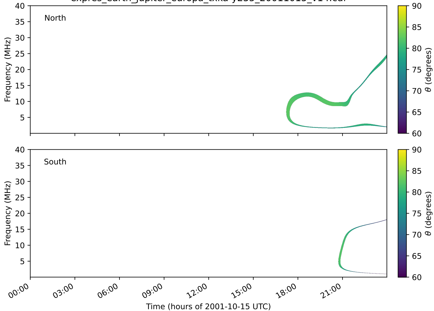
expres_earth_jupiter_europa_txka-y235_20011015_v14.cdf
