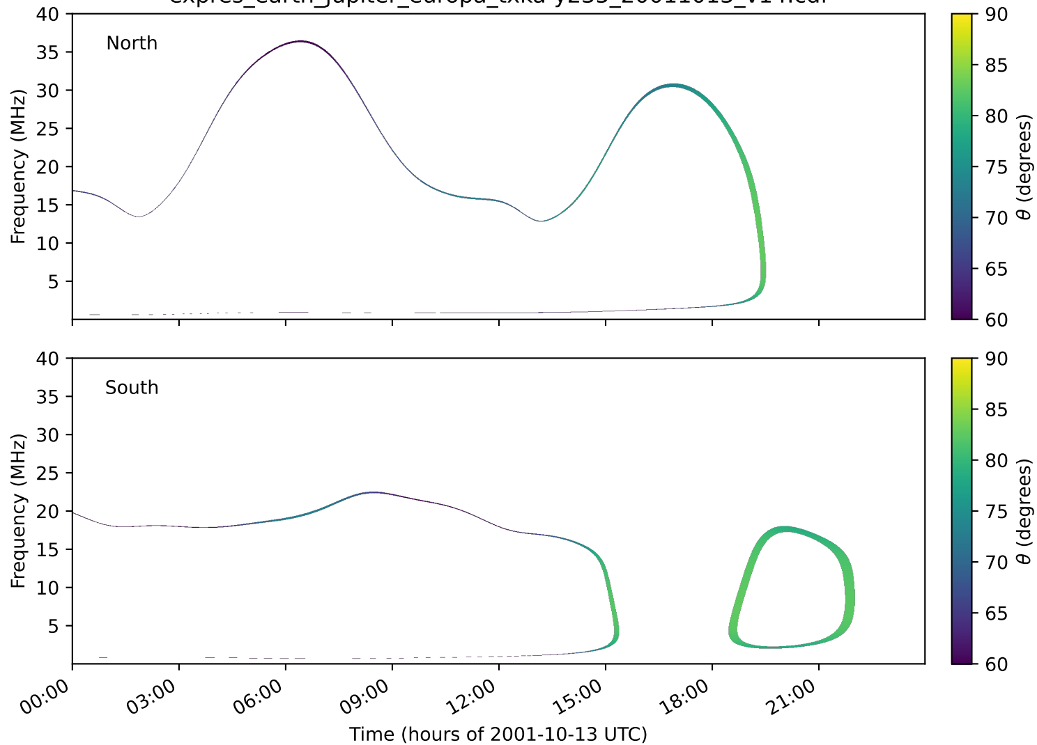
expres_earth_jupiter_europa_txka-y235_20011013_v14.cdf
