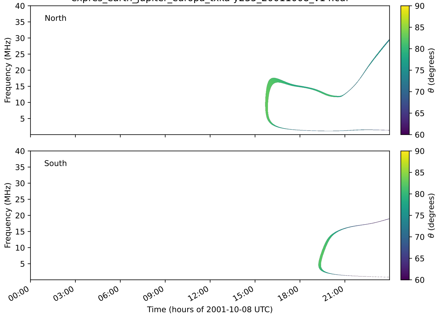
expres_earth_jupiter_europa_txka-y235_20011008_v14.cdf
