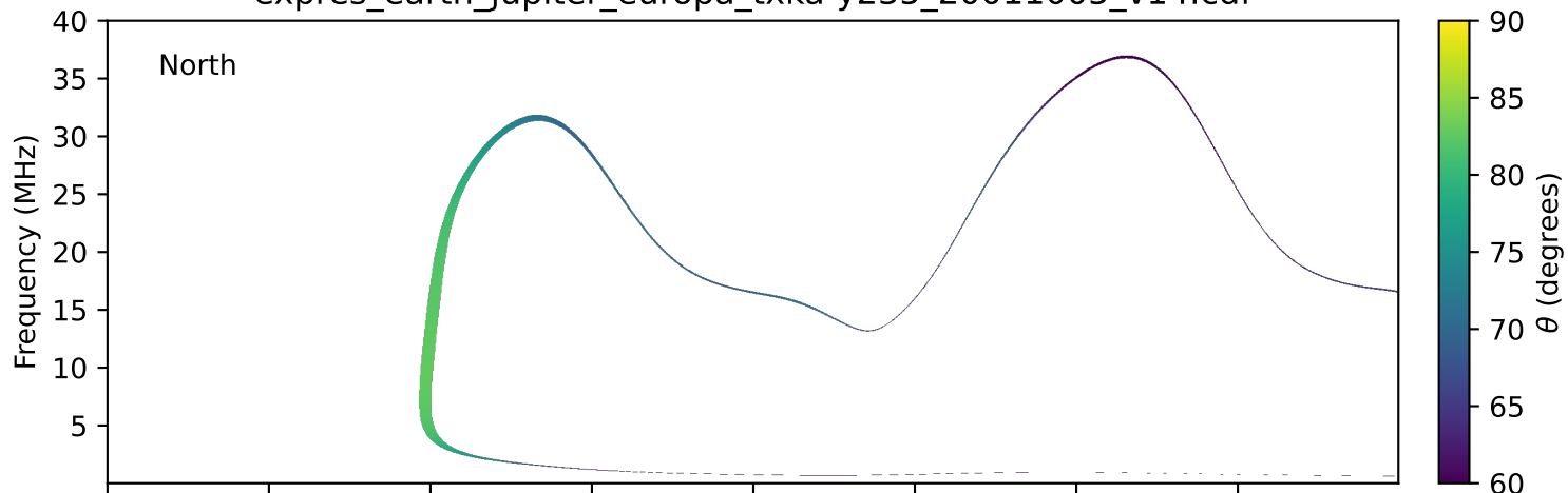
expres_earth_jupiter_europa_txka-y235_20011005_v14.cdf
