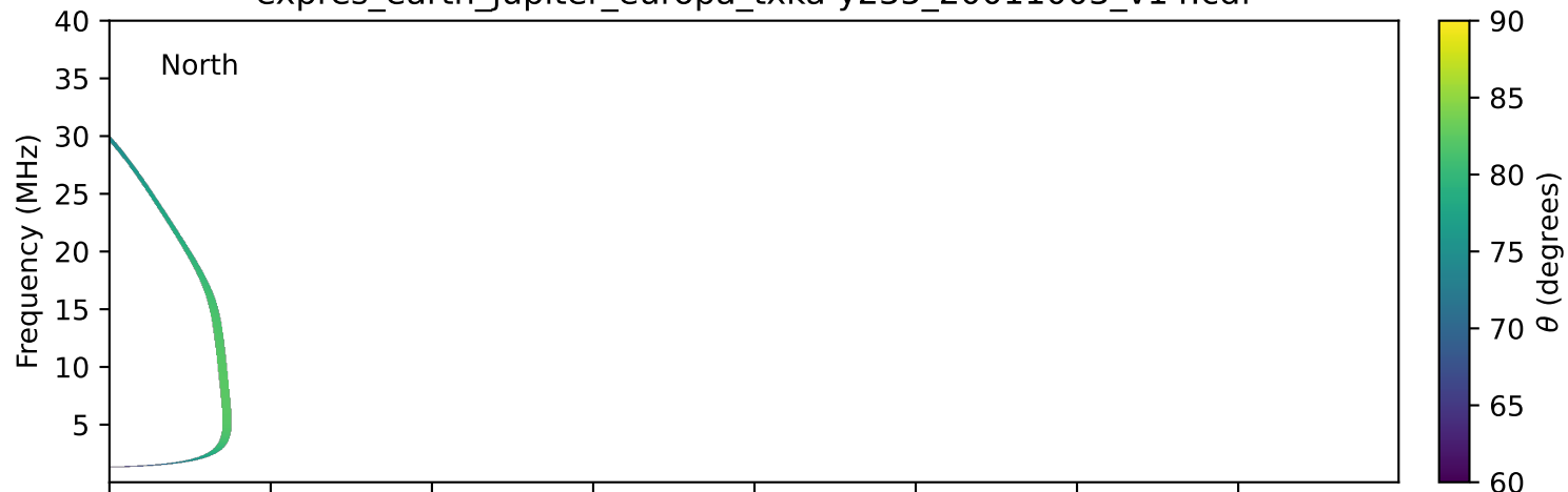
expres_earth_jupiter_europa_txka-y235_20011003_v14.cdf
