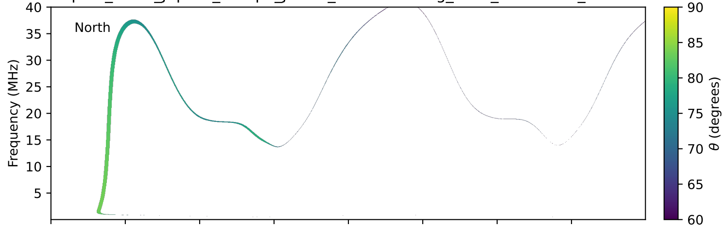
expres_earth_jupiter_europa_jrm33_lossc-wid1deg_3kev_20011030_v11.cdf
