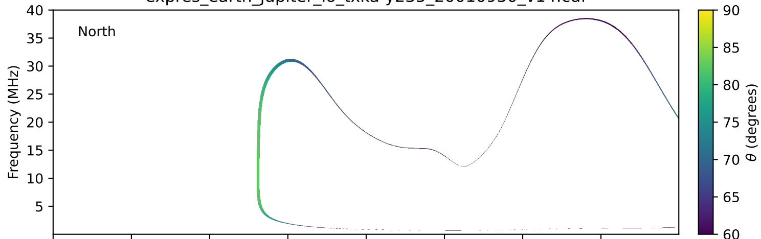
expres_earth_jupiter_io_txka-y235_20010930_v14.cdf
