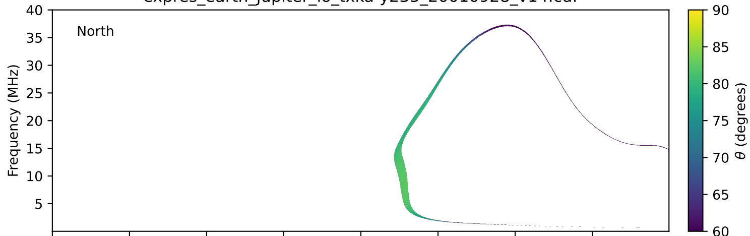
expres_earth_jupiter_io_txka-y235_20010928_v14.cdf
