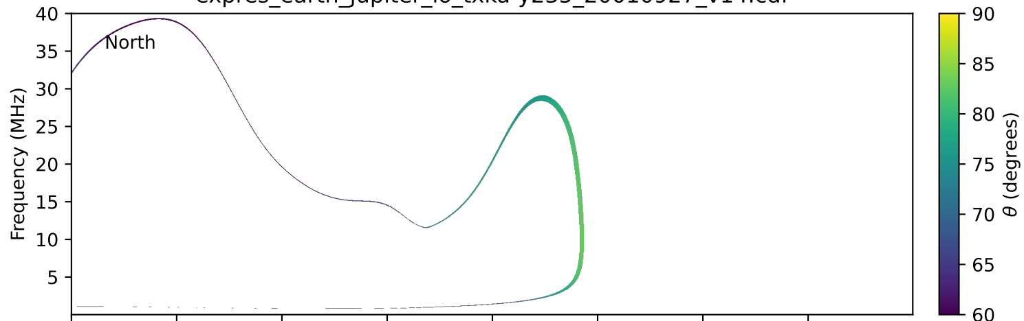
expres_earth_jupiter_io_txka-y235_20010927_v14.cdf
