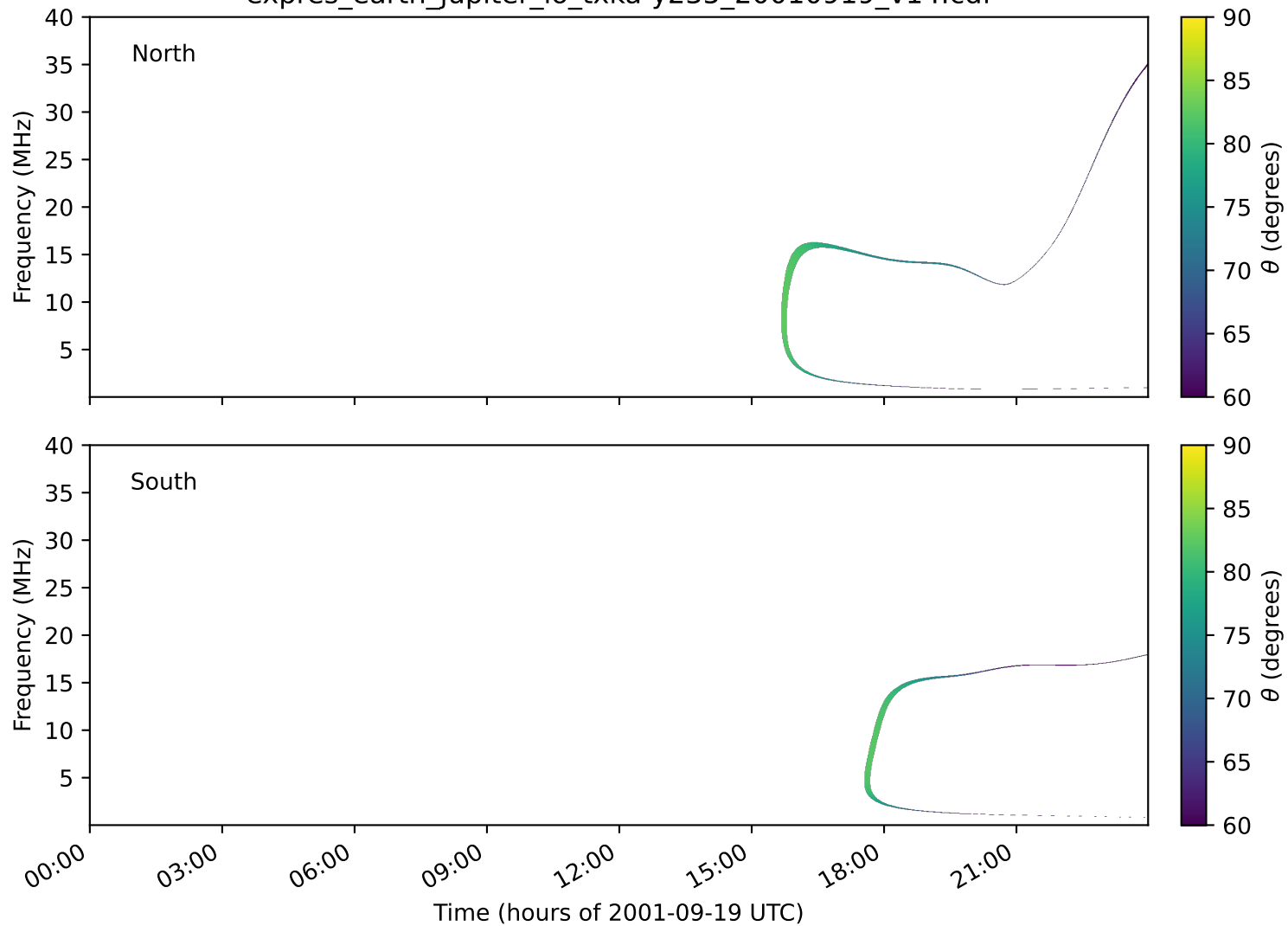
expres_earth_jupiter_io_txka-y235_20010919_v14.cdf
