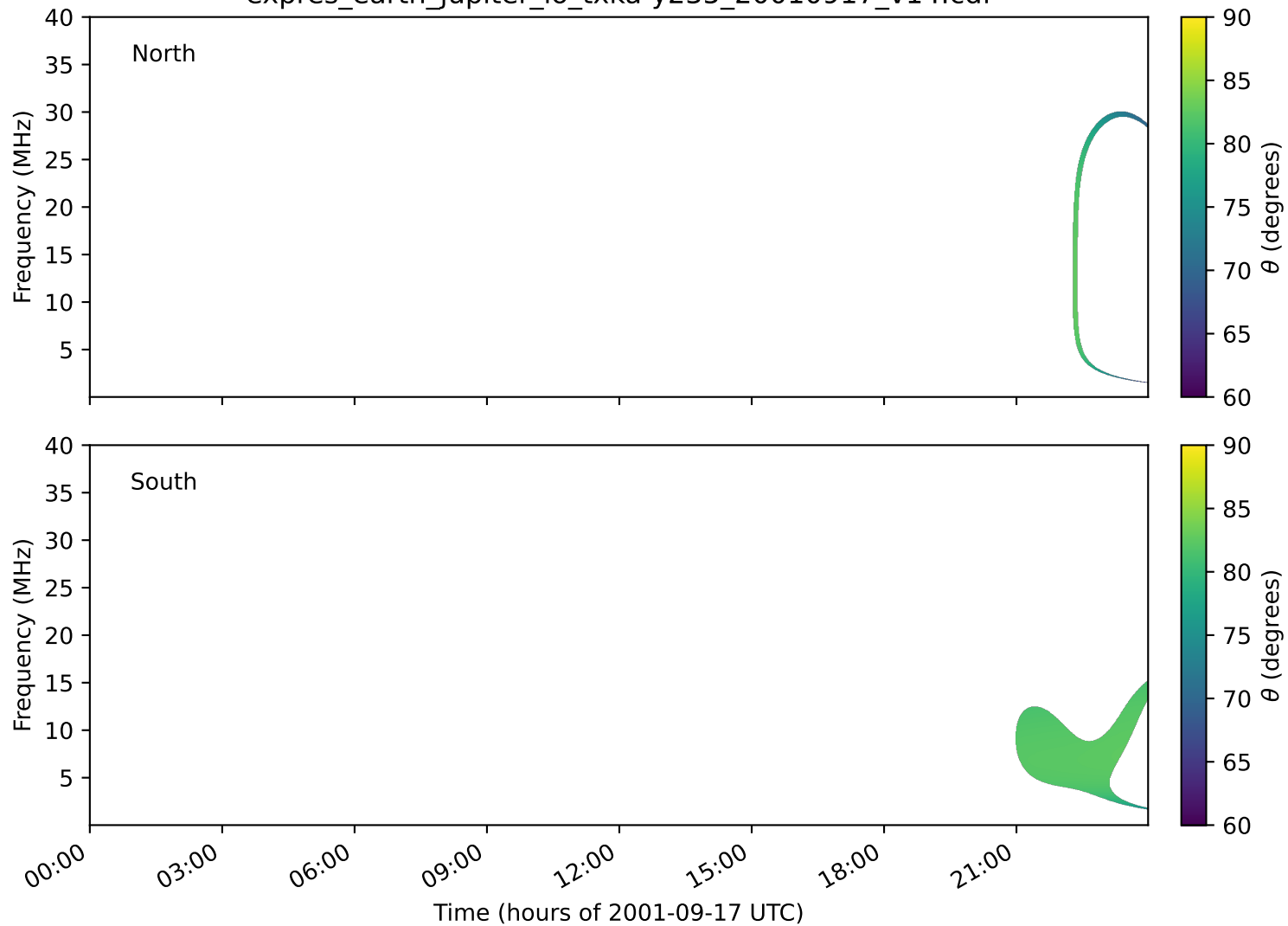
expres_earth_jupiter_io_txka-y235_20010917_v14.cdf
