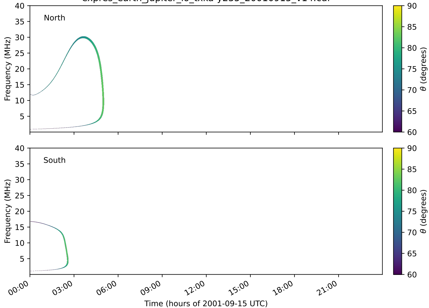
expres_earth_jupiter_io_txka-y235_20010915_v14.cdf
