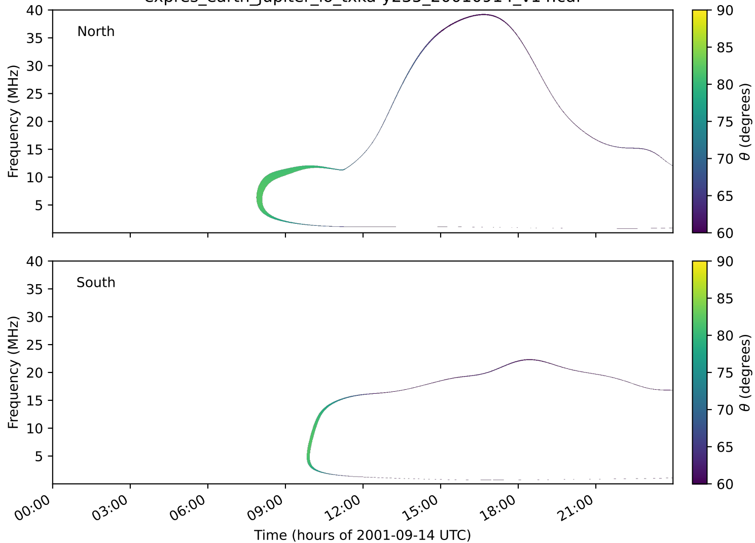
expres_earth_jupiter_io_txka-y235_20010914_v14.cdf
