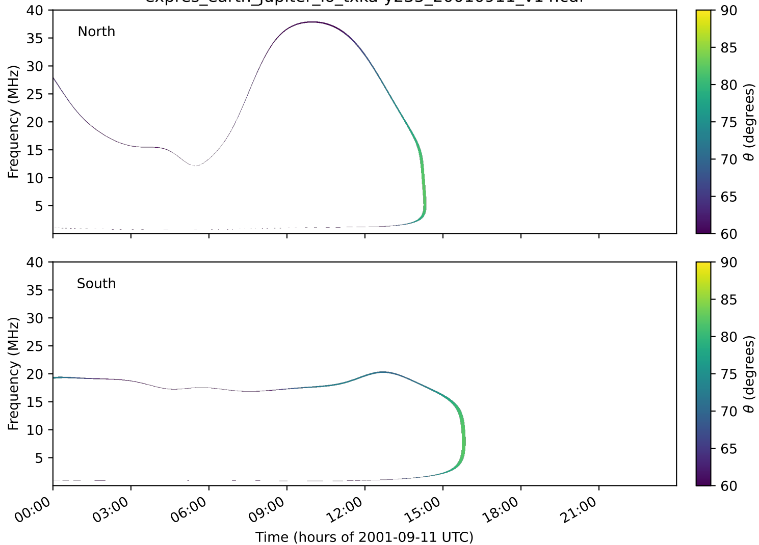
expres_earth_jupiter_io_txka-y235_20010911_v14.cdf
