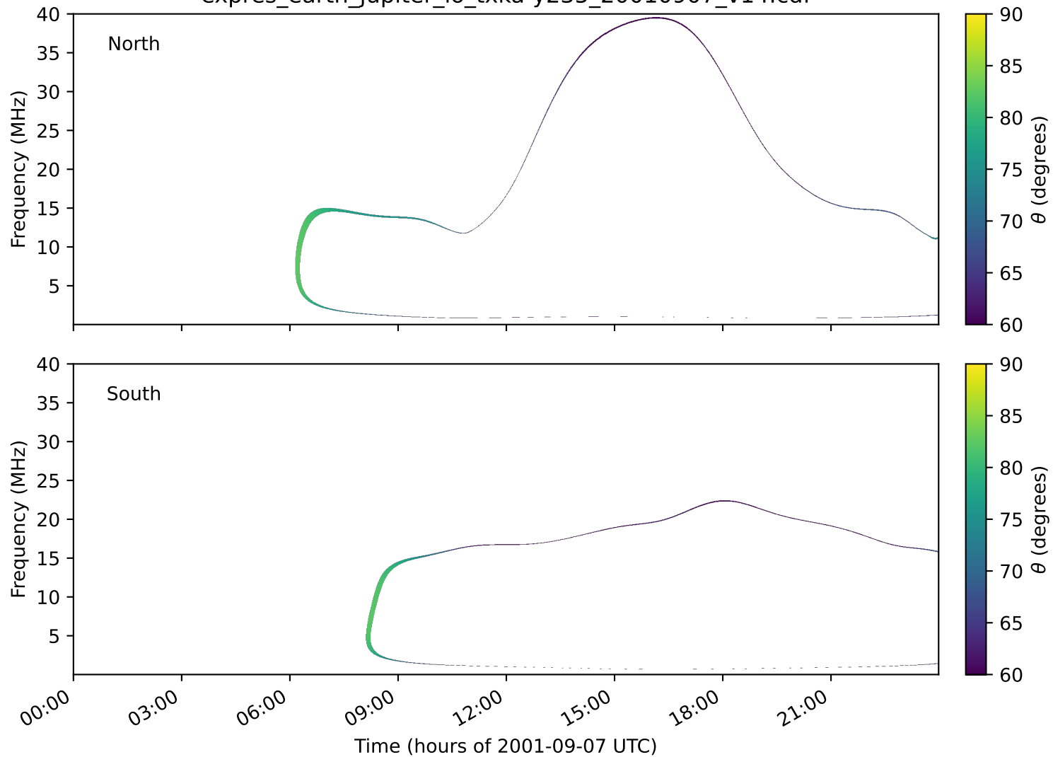
expres_earth_jupiter_io_txka-y235_20010907_v14.cdf
