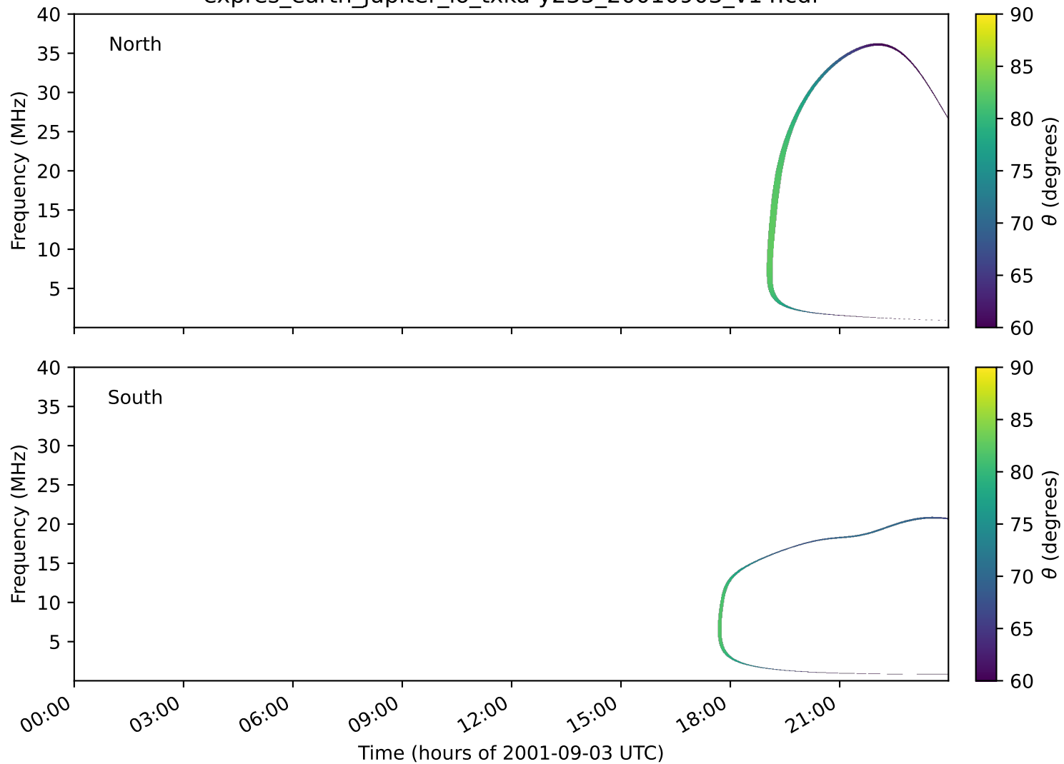
expres_earth_jupiter_io_txka-y235_20010903_v14.cdf
