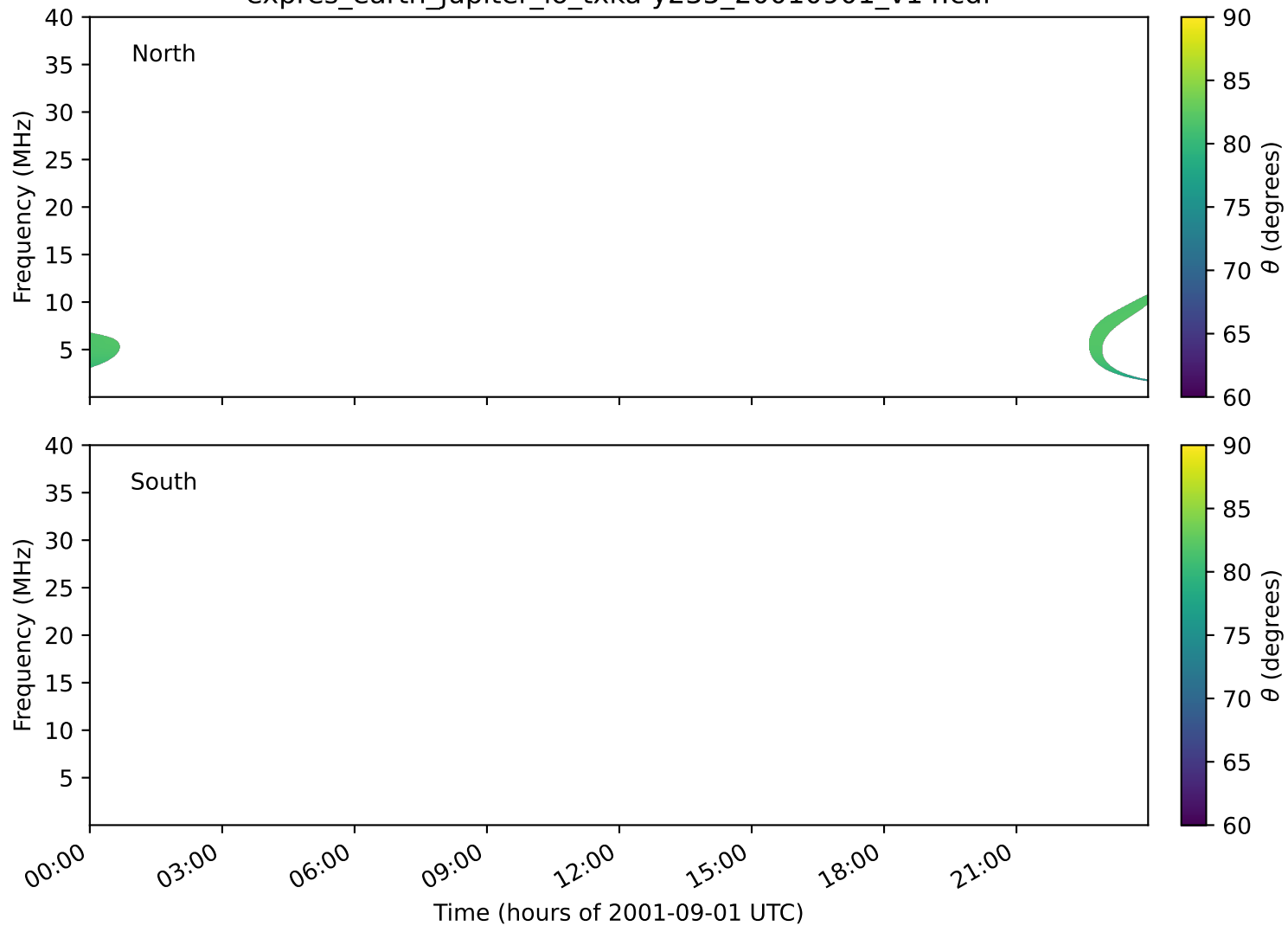
expres_earth_jupiter_io_txka-y235_20010901_v14.cdf
