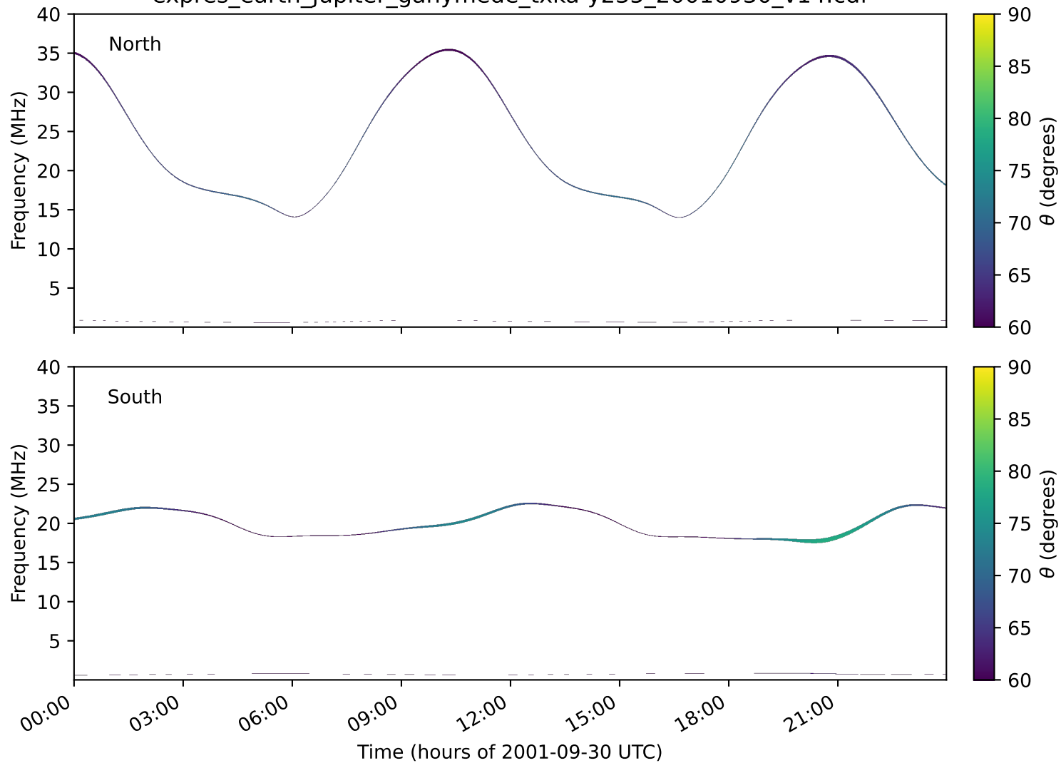
expres_earth_jupiter_ganymede_txka-y235_20010930_v14.cdf
