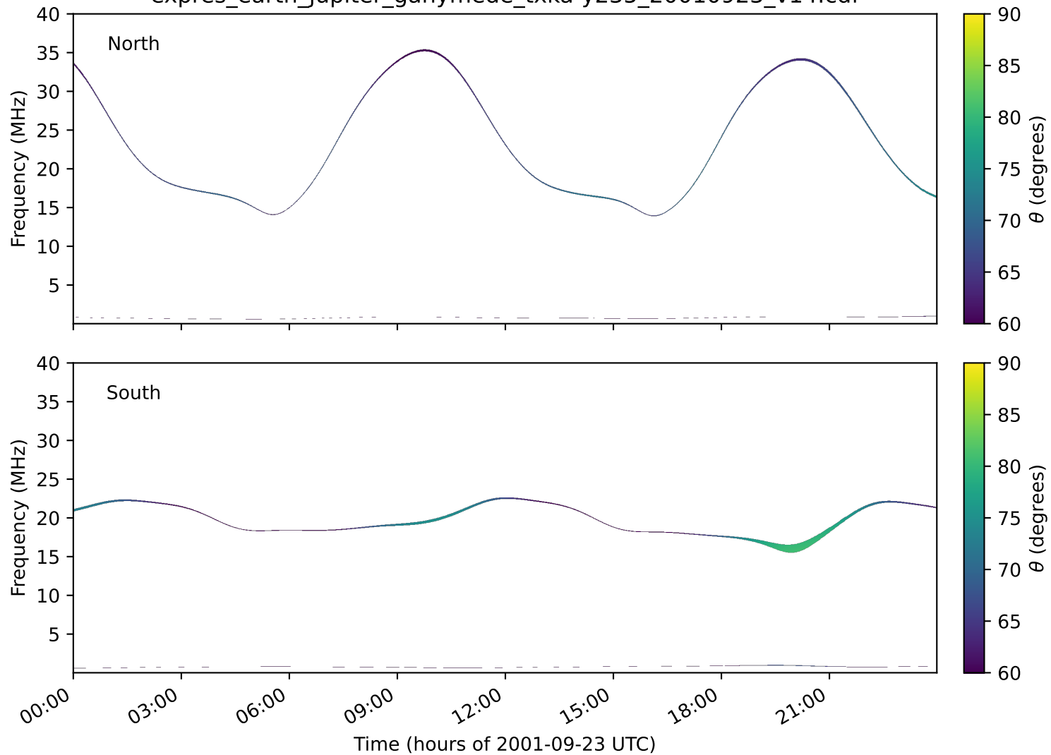
expres_earth_jupiter_ganymede_txka-y235_20010923_v14.cdf
