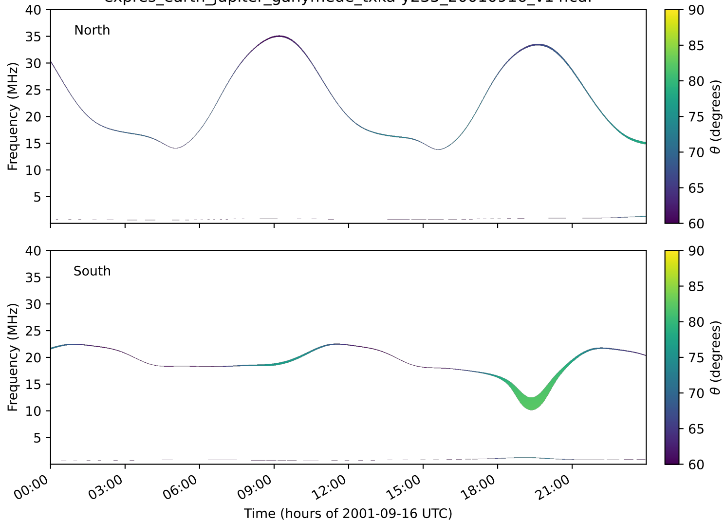
expres_earth_jupiter_ganymede_txka-y235_20010916_v14.cdf
