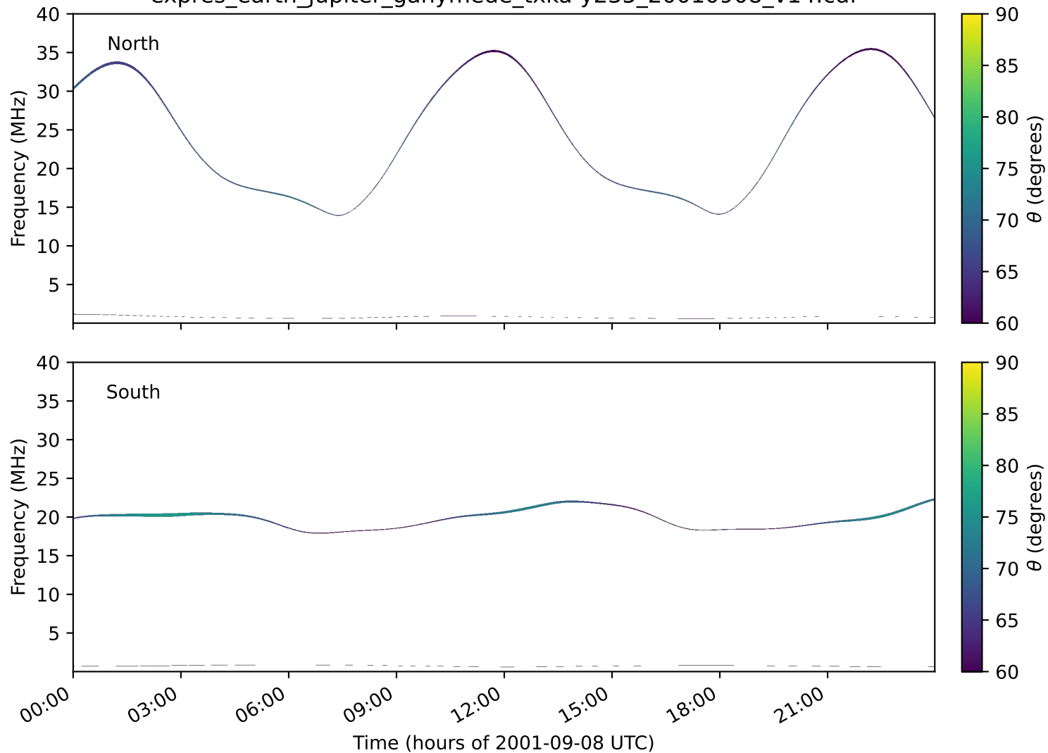
expres_earth_jupiter_ganymede_txka-y235_20010908_v14.cdf
