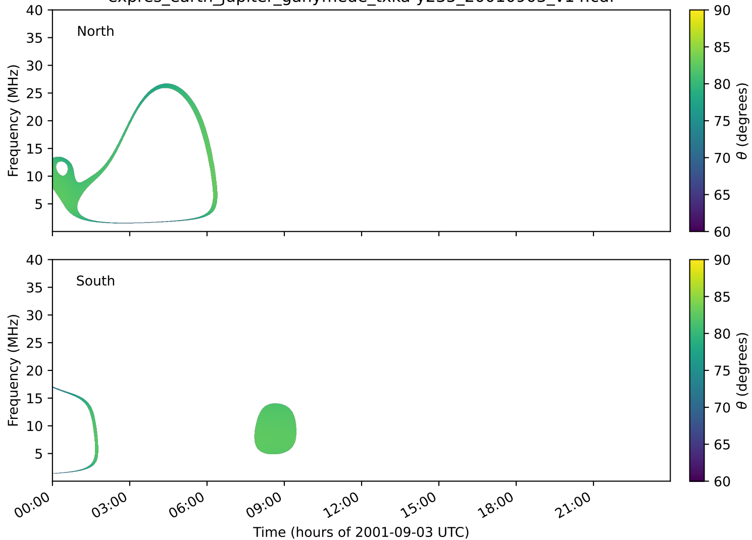
expres_earth_jupiter_ganymede_txka-y235_20010903_v14.cdf
