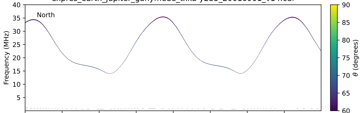
expres_earth_jupiter_ganymede_txka-y235_20010901_v14.cdf
