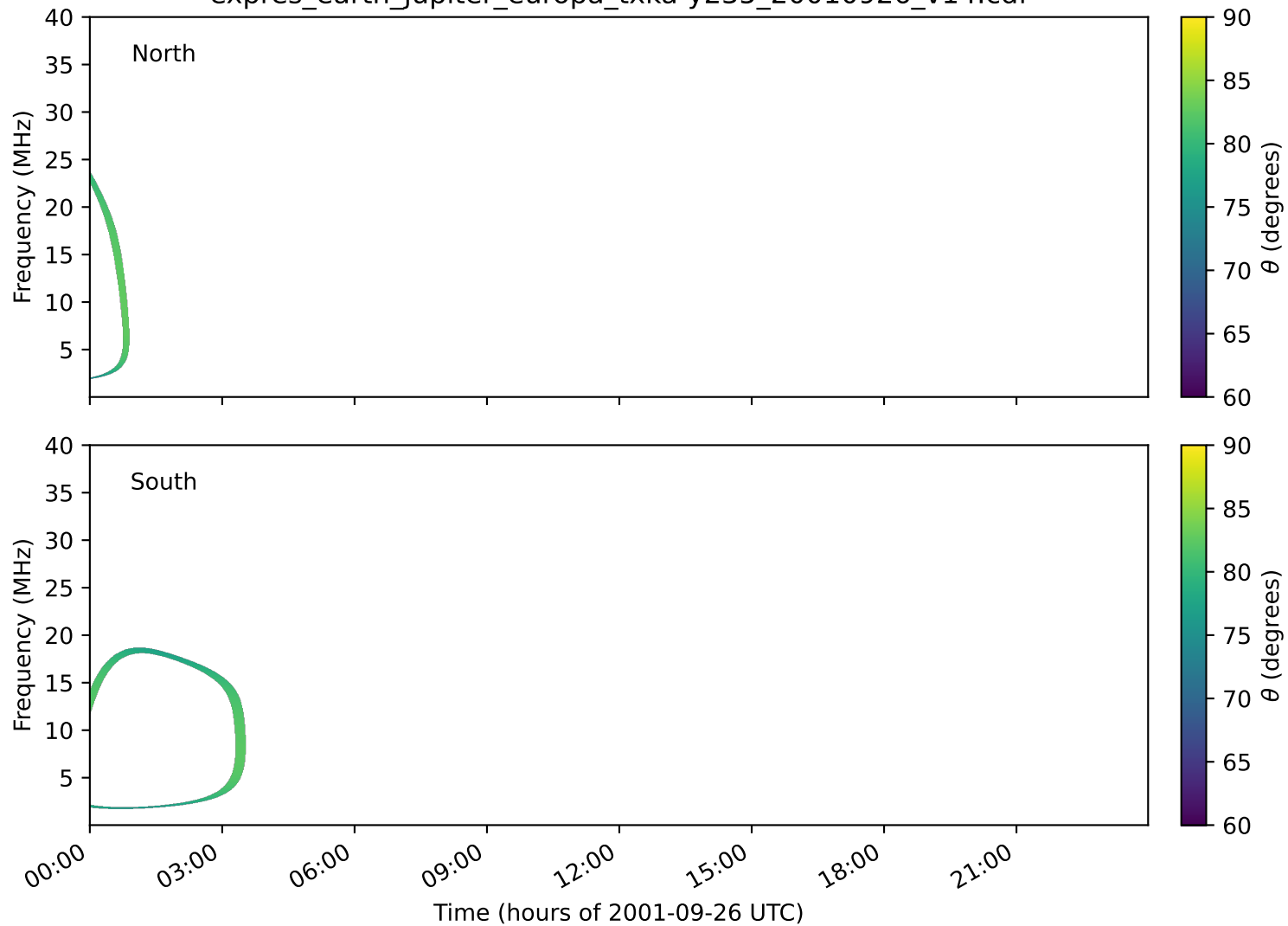
expres_earth_jupiter_europa_txka-y235_20010926_v14.cdf
