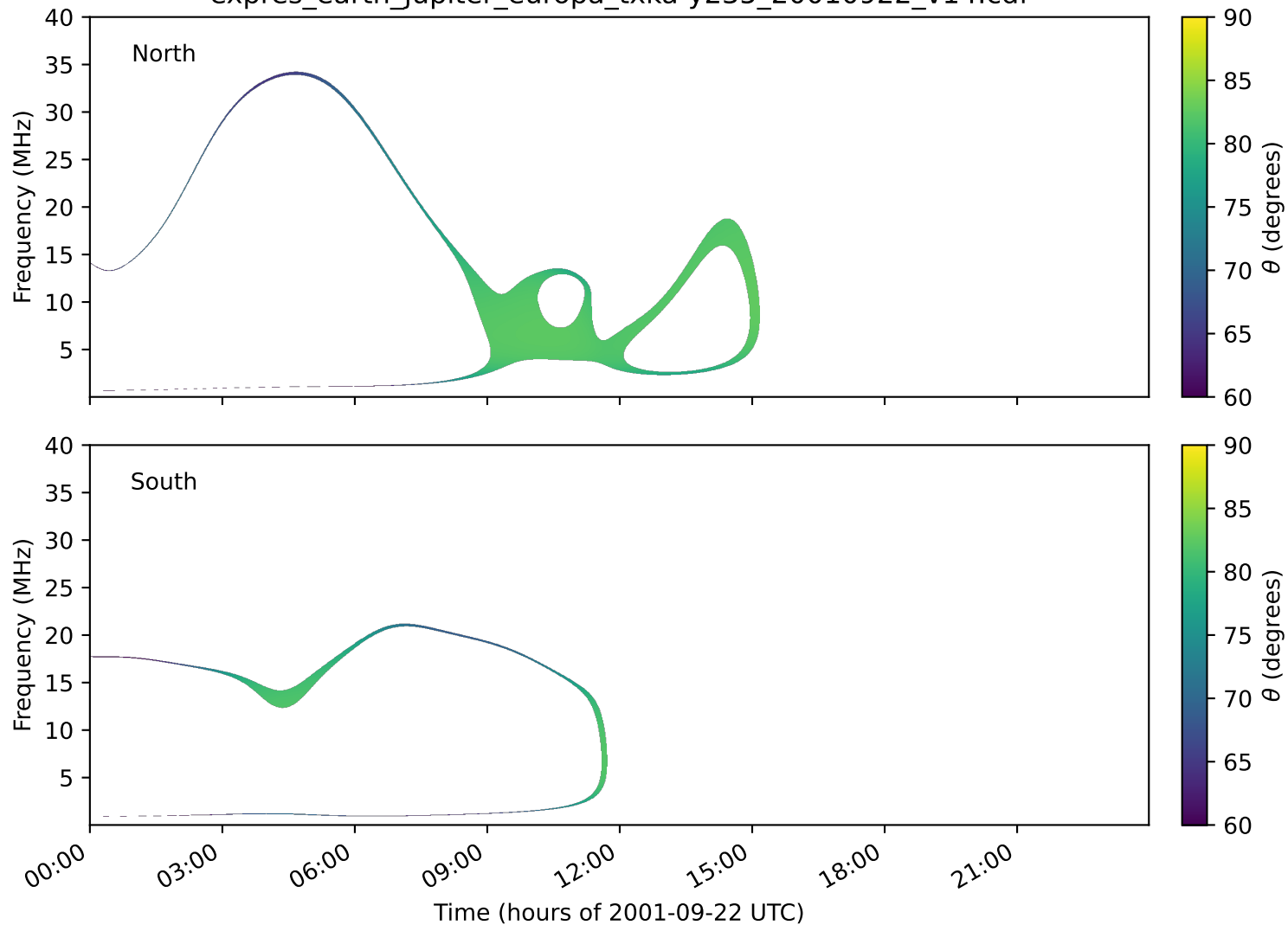
expres_earth_jupiter_europa_txka-y235_20010922_v14.cdf
