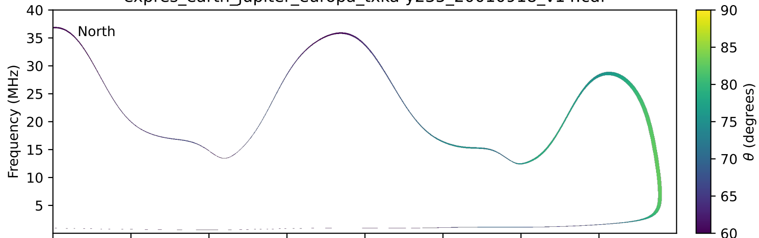
expres_earth_jupiter_europa_txka-y235_20010918_v14.cdf
