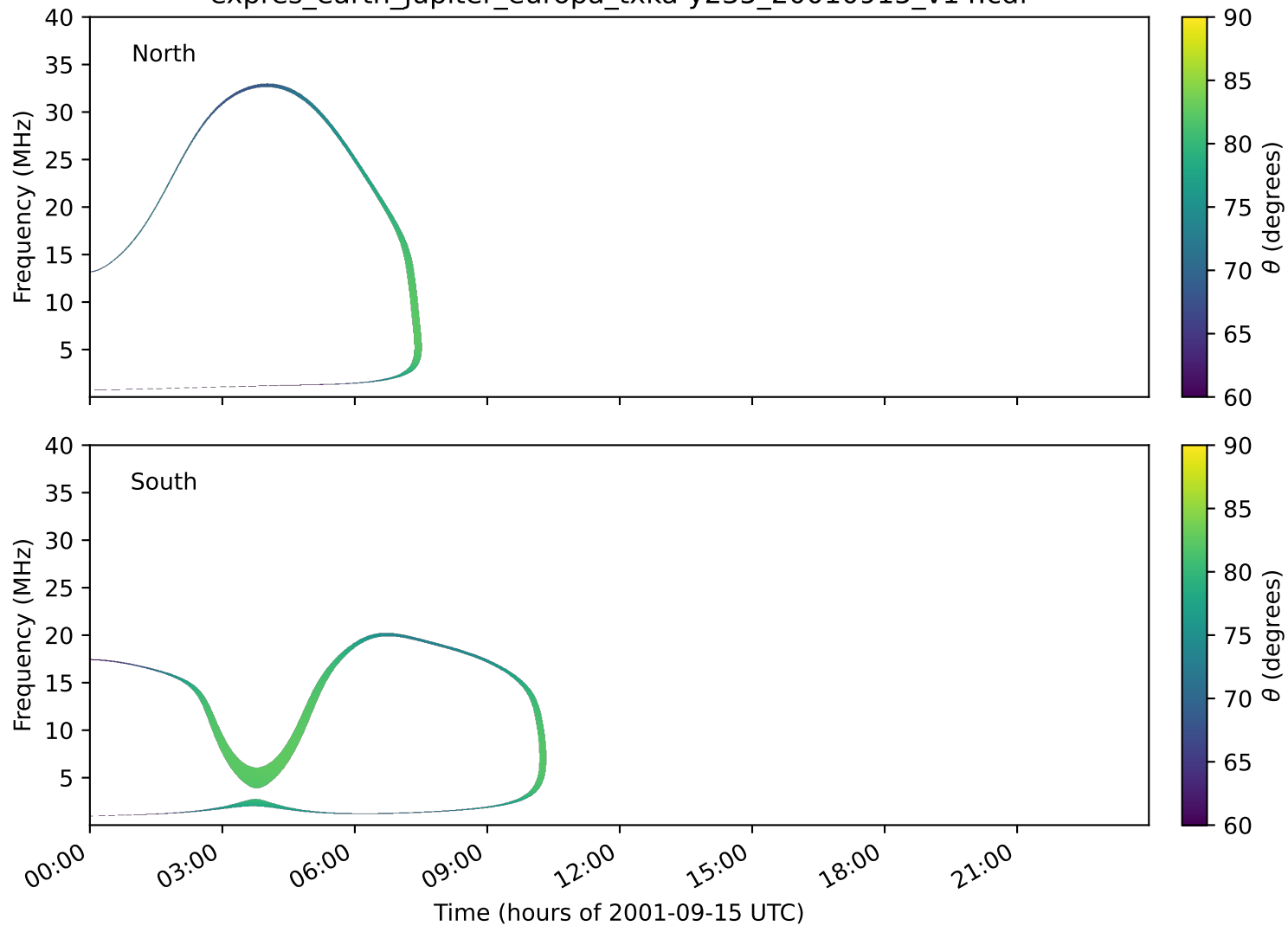
expres_earth_jupiter_europa_txka-y235_20010915_v14.cdf
