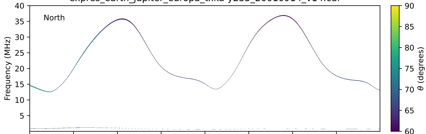
expres_earth_jupiter_europa_txka-y235_20010914_v14.cdf
