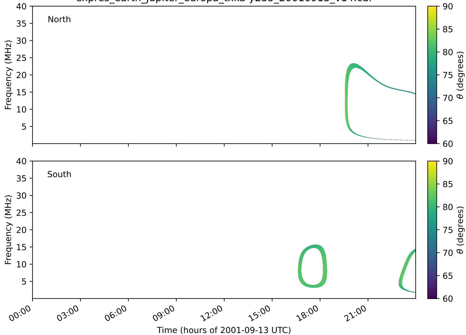
expres_earth_jupiter_europa_txka-y235_20010913_v14.cdf
