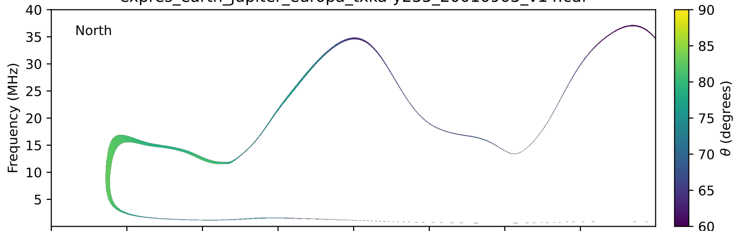
expres_earth_jupiter_europa_txka-y235_20010903_v14.cdf
