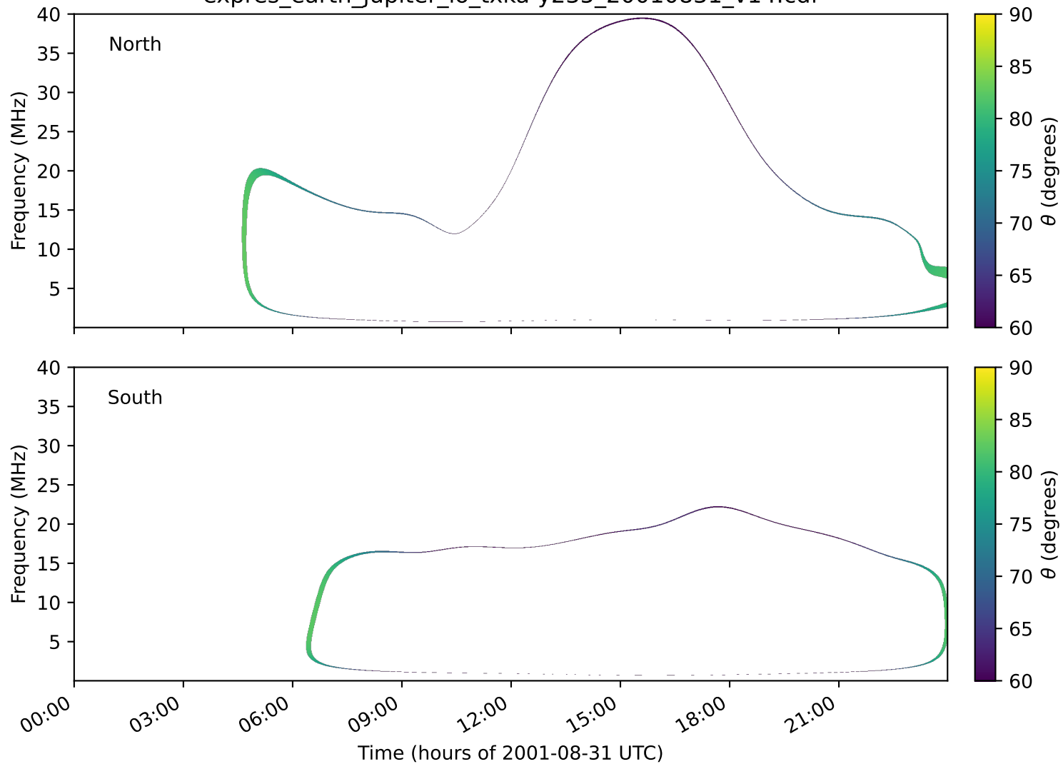
expres_earth_jupiter_io_txka-y235_20010831_v14.cdf
