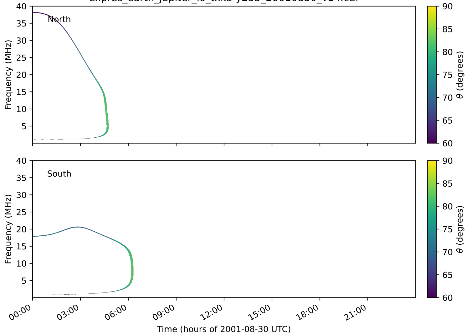
expres_earth_jupiter_io_txka-y235_20010830_v14.cdf
