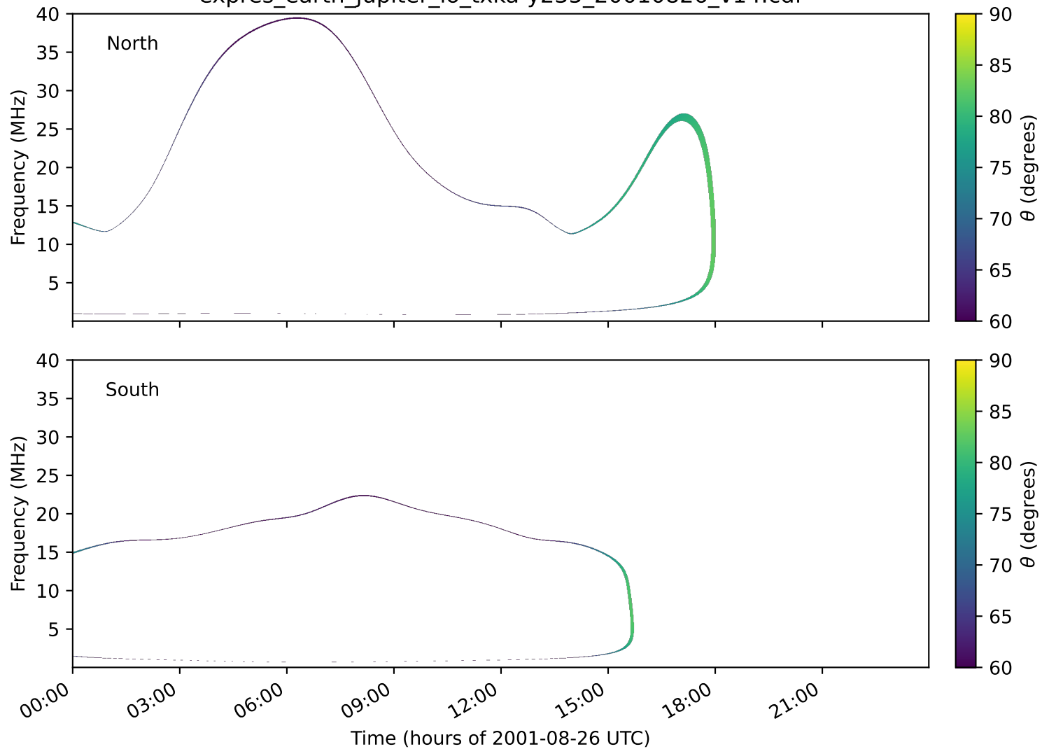
expres_earth_jupiter_io_txka-y235_20010826_v14.cdf
