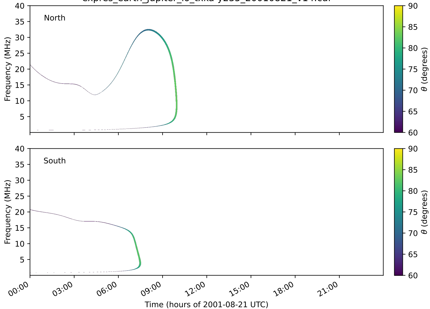
expres_earth_jupiter_io_txka-y235_20010821_v14.cdf
