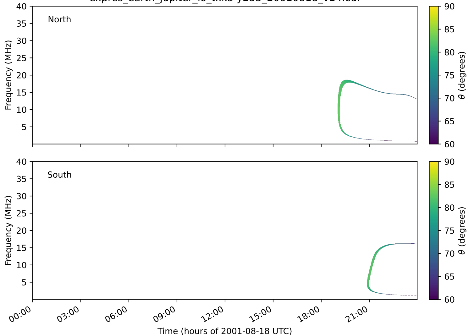
expres_earth_jupiter_io_txka-y235_20010818_v14.cdf
