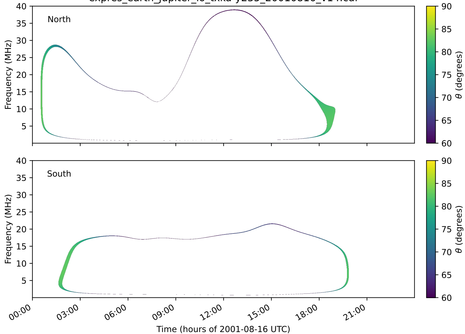
expres_earth_jupiter_io_txka-y235_20010816_v14.cdf
