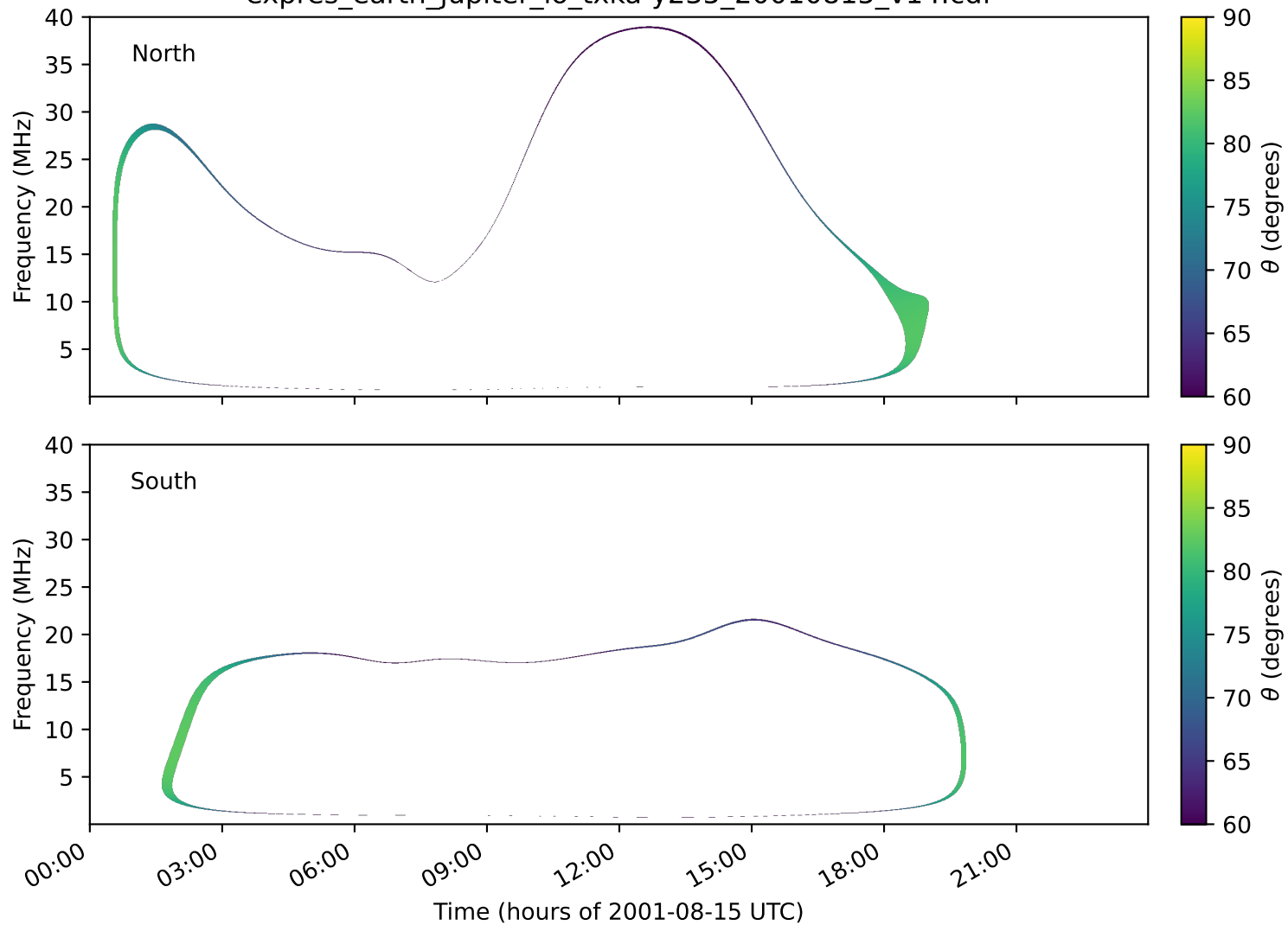
expres_earth_jupiter_io_txka-y235_20010815_v14.cdf
