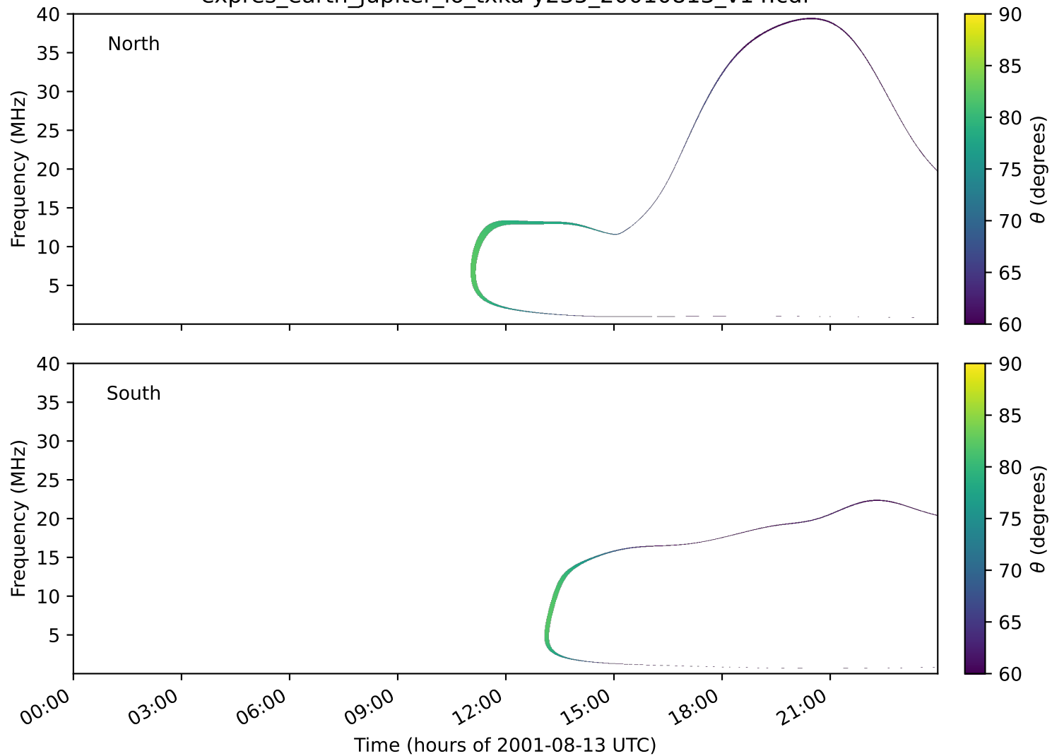
expres_earth_jupiter_io_txka-y235_20010813_v14.cdf
