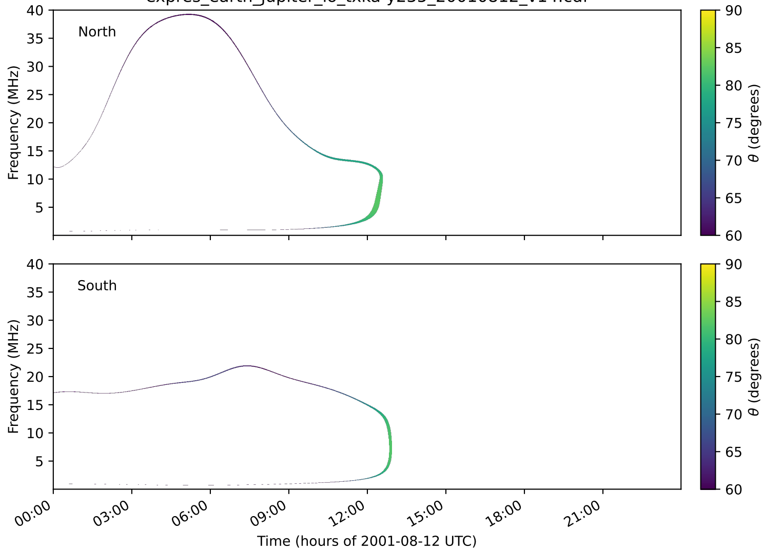
expres_earth_jupiter_io_txka-y235_20010812_v14.cdf
