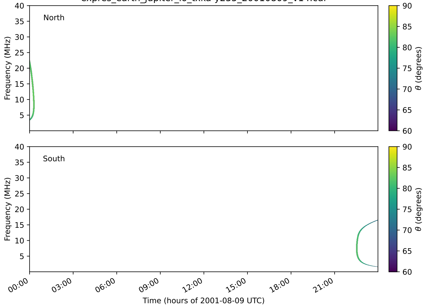
expres_earth_jupiter_io_txka-y235_20010809_v14.cdf
