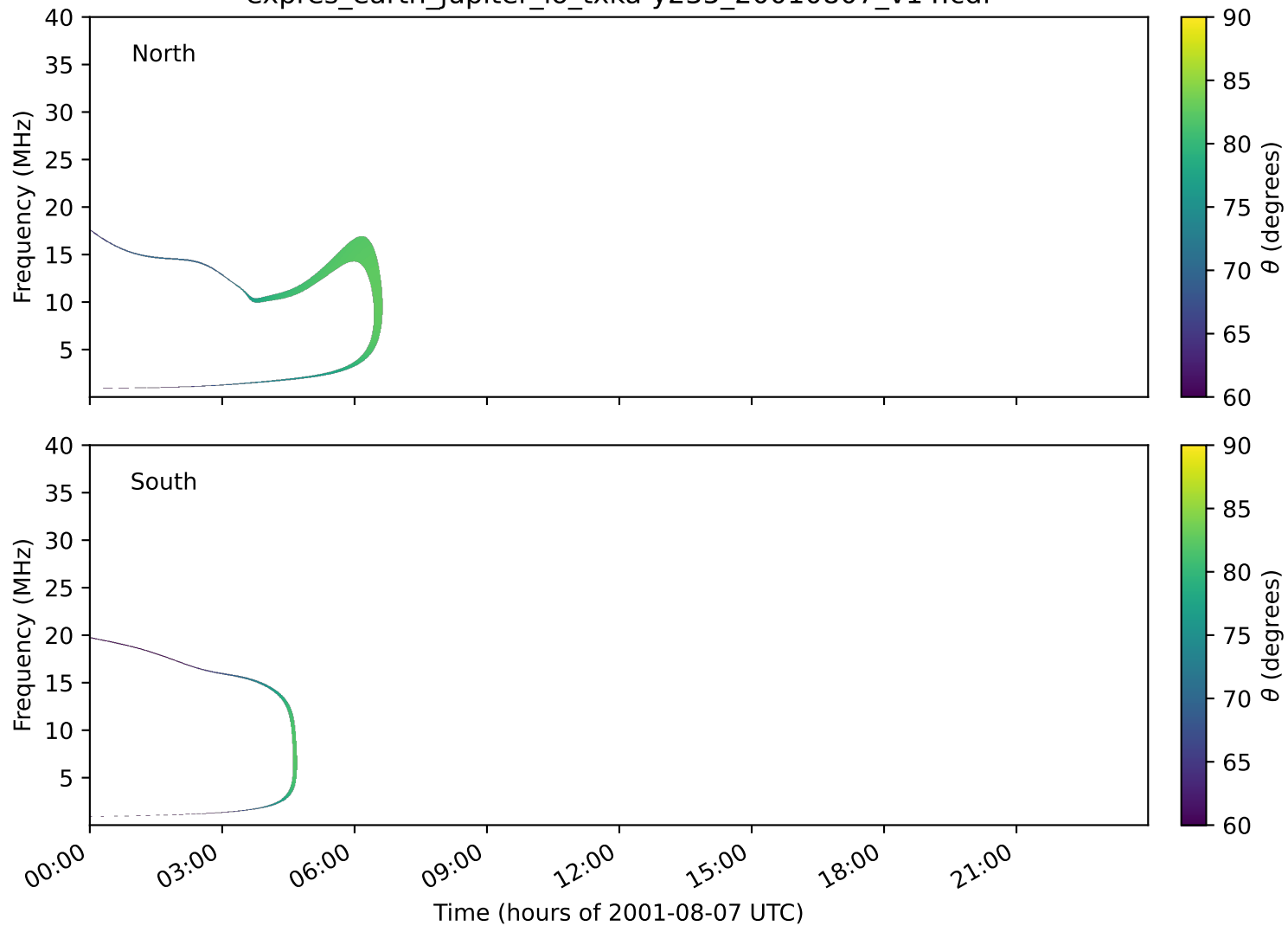
expres_earth_jupiter_io_txka-y235_20010807_v14.cdf
